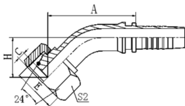
20442 20442-T 45°METRIC FEMALE 24°CONE O-RING L.T.
