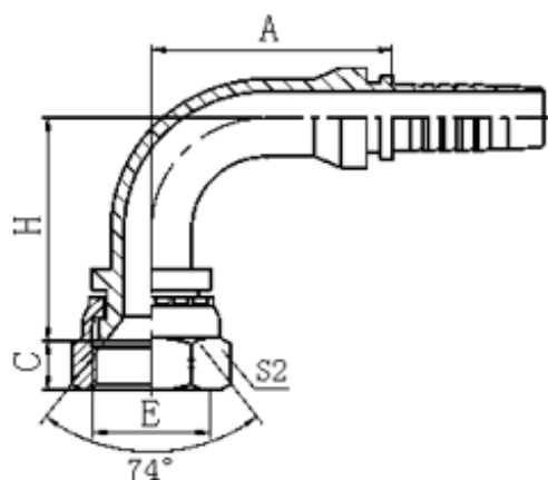
26792, 26792W 90° JIC 74° 90° JIC FEMALE 74° CONE SEAT
