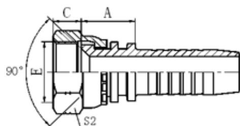
27811 SAE FEMALE 90° CONE SEAT
