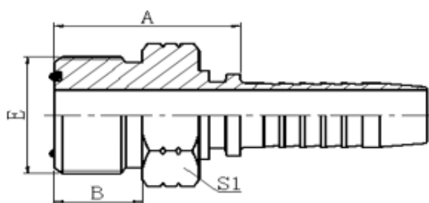
14211 ORFS MALE O-RING SEAL
