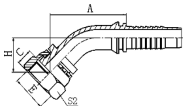
20242 20242-T 45° GB METRIC FEMALE FLAT SEAT
