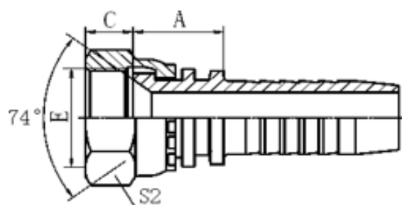
20711 20711-T GB METRIC FEMALE 74° CONE SEAT
