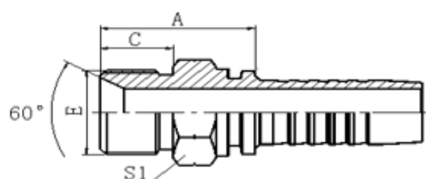
12611 BSP MALE 60° CONE SEAT
