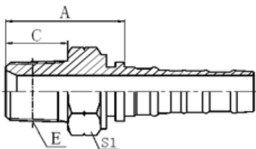
13013-SP BSPT MALE
