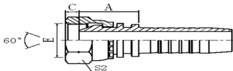
2261, 22611 -T, 22611-W BSP FEMALE 60° CONE
