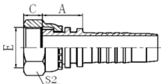
20212 20212-T GB METRIC FEMALE FLAT SEAT
