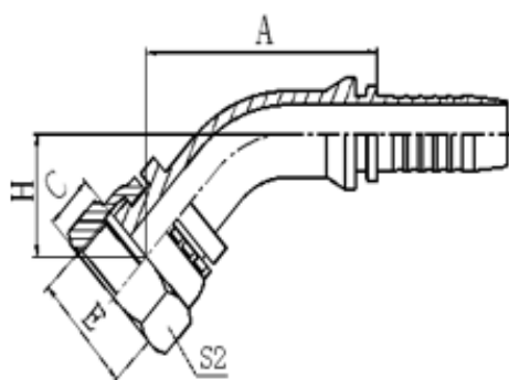
20231 20231-T 30° METRIC FEMALE FLAT SEAT REF. GB/T 9065.3
