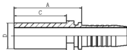
50011 METRIC STANDPIPE STRAIGHTDIN 2353
