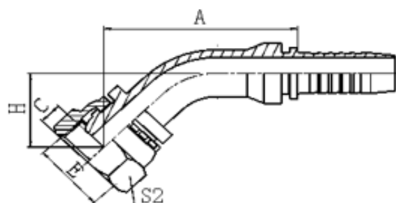
20141, 20141-T 45° METRIC FEMALE MULTISEAL
